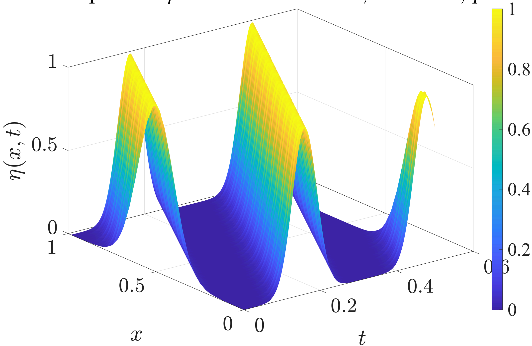
Surface plot of \eta with \Delta t = 0.01 ms, h = 0.10 , p = 4 .
